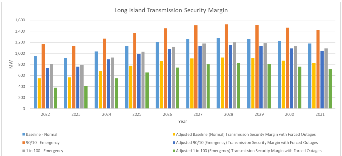
Figure 16: Long Island Transmission Security Margin
